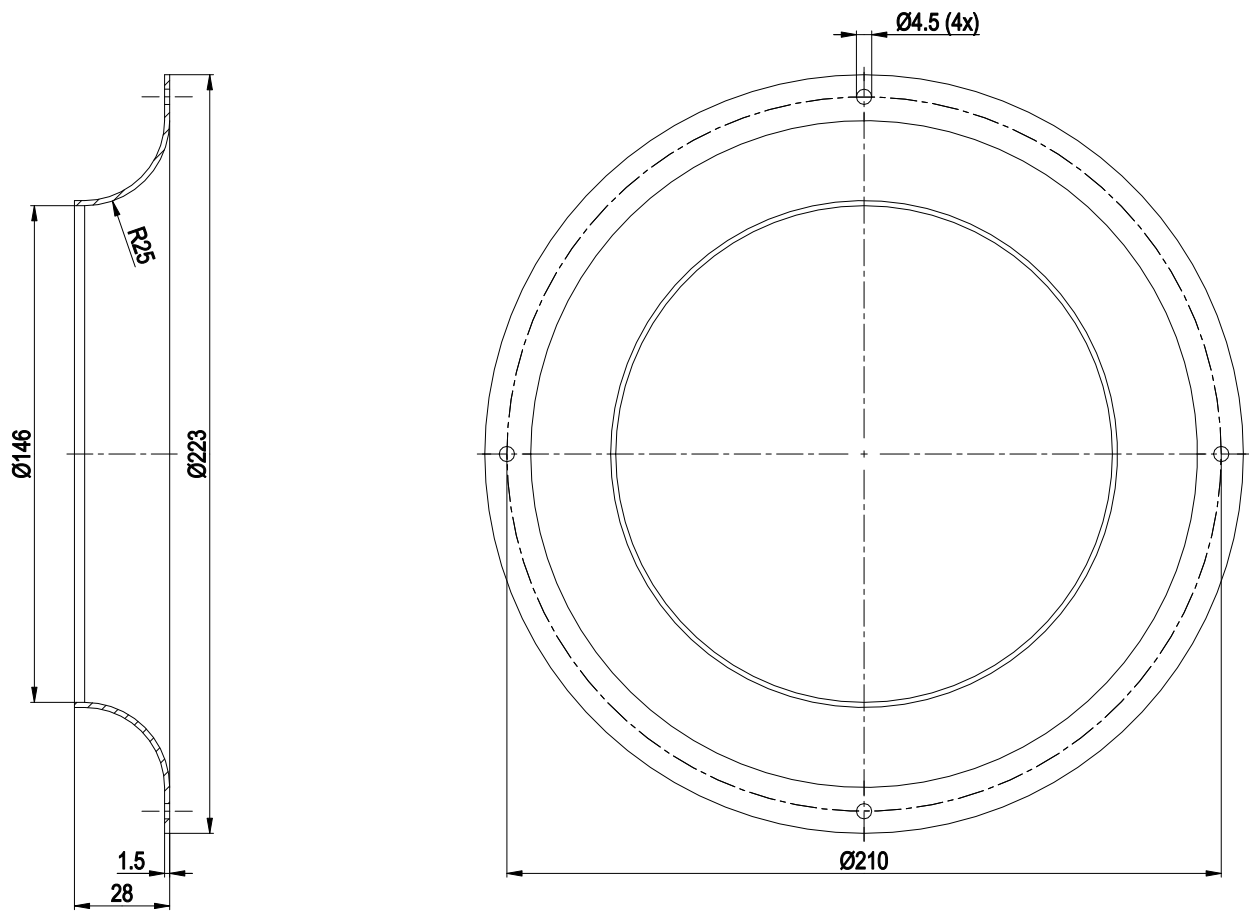
Inlet ring 96358-2-4013
