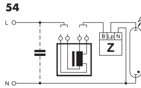
Superimposed ignition of HS and HI lamps (ballasts with two alternative voltage and power tapping points)
